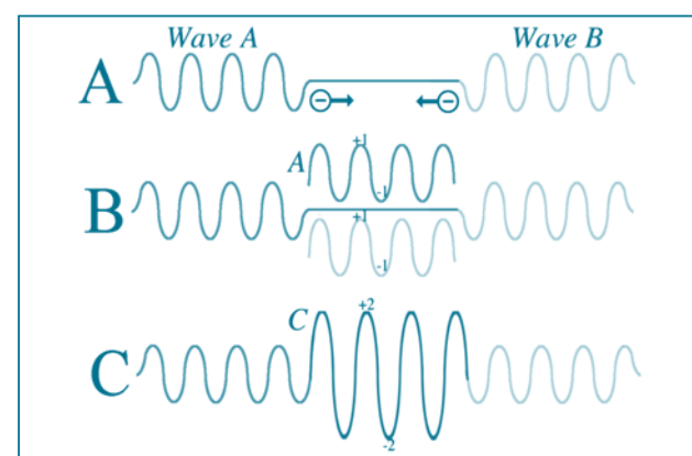
Figure 2: Constructive Interference
