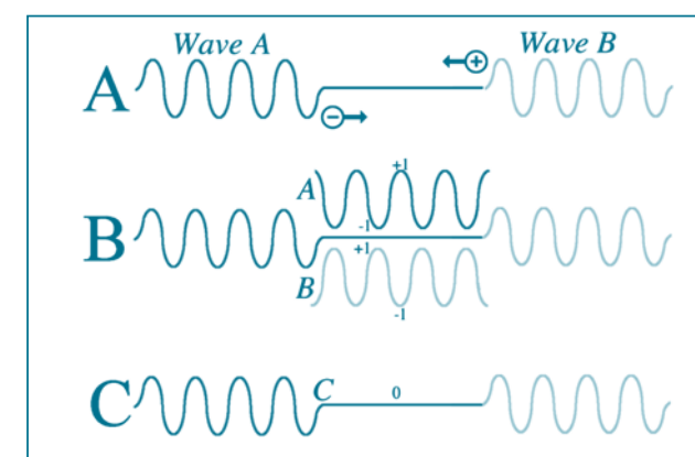
Figure 3: Destructive Interference
